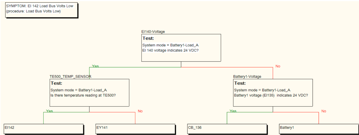
Figure 4. An auto-generated diagnostic tree for a voltage anomaly indicated at sensor EI142 (EI142 in Fig. 2)
