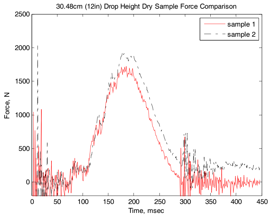
Figure 22. Force comparison of 30.48 cm (12in) drop height dry testing.
