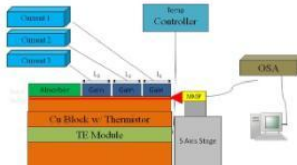
Figure 3. Schematic of the improved segmented contact method set up used to measure the gain. A multimode fiber (MMF) is used to collect light from the device. Absorption measurements can also be performed on the same set up by applying a reverse bias voltage to section L_2 . Data acquisition is performed by LabView and IGOR Pro software packages.
