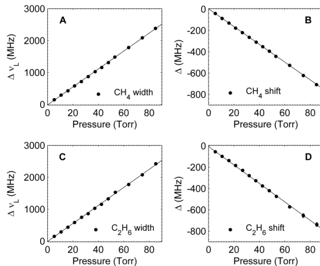
Figure 7. Lorentzian line width \Delta \nu_L and shift \Delta of the Rb D2 transition obtained from measured absorption spectra as a function of methane ( \text{CH}_4 ) and ethane ( \text{C}_2\text{H}_6 ) buffer gas pressure A&B and C&D respectively ( T=314 K). Experimental data (dots ●), solid line is weighted linear fit.
