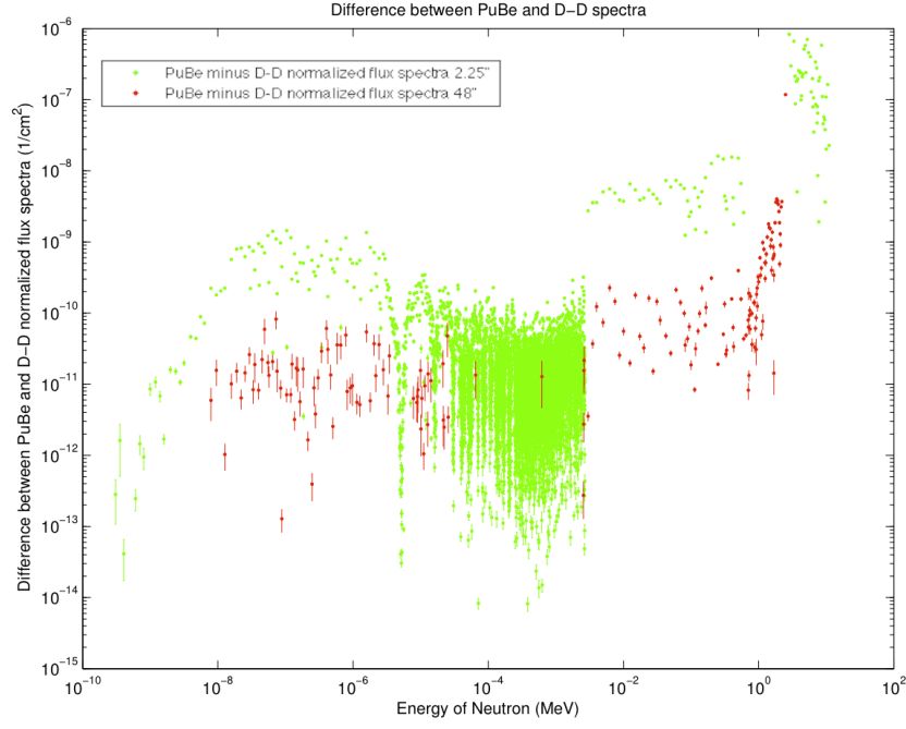
Figure 16. Relative difference of PuBe to D-D MCNP spectra.
