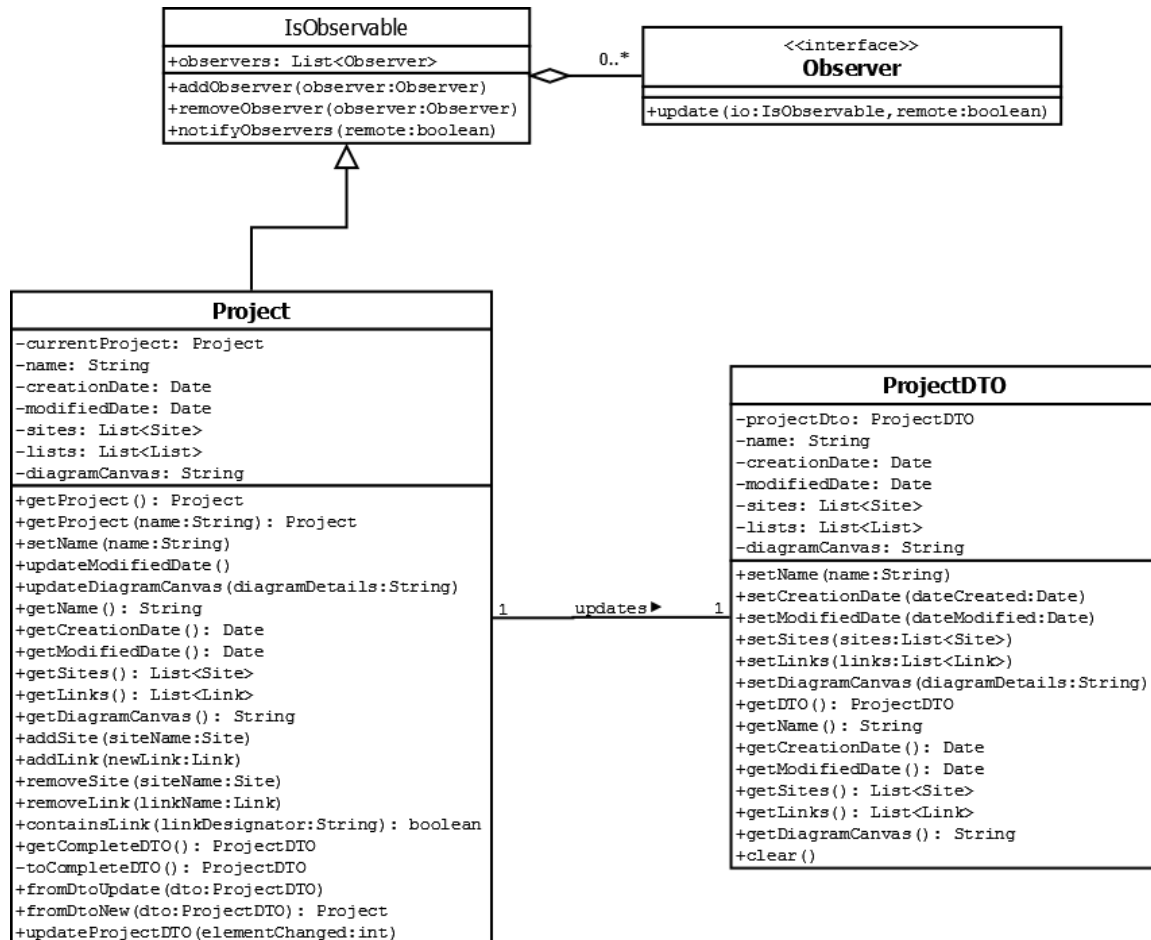
Figure 9. ProjectDTO
