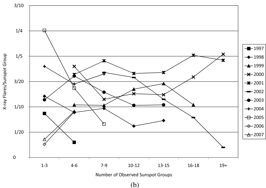
Figure 10 Total number of (a) H \alpha flares and (b) X-ray flares divided by the total number of sunspot groups in each daily total sunspot group category. Values are shown only when a sunspot count category had at least 50 sunspot groups.
