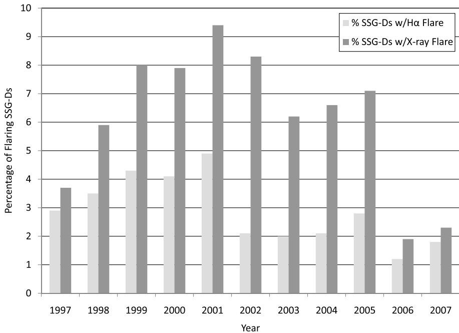
Figure 2 Percentages of SSG-Ds with at least one H \alpha flare and of SSG-Ds with at least one X-ray flare as computed from the flaring and total SSG-D counts in Figure 1.
