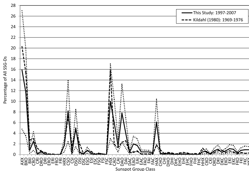
Figure 4 Frequency distribution (percent) of SSG-Ds by known McIntosh (1990) classification from the current study for the years 1997–2007 compared to the same found by Kildahl (1980) for the years 1969–1976. The dotted curves represent the upper and lower bounds of the values from the current study when accounting for the uncertainty in assigning the sunspot group class to the observed sunspot groups.
