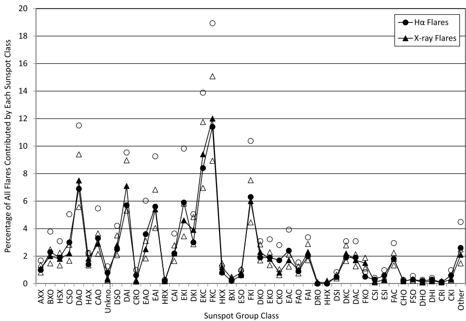
Figure 7 Percentage of all flares that originated from each sunspot group class. The order of the classes left to right is by total number of SSG-Ds over all years as in Figure 3. Only the classes with at least 0.1% of the total number of SSG-Ds with known classification are shown, along with the percentage flare contribution of SSG-Ds of unknown class. The class designated “Other” includes the percentage flare contributions from all sunspot group classes with less than 0.1% of SSG-Ds with known classification. Open symbols indicate uncertainty of the flare assignment to sunspot groups as in Figure 5.
