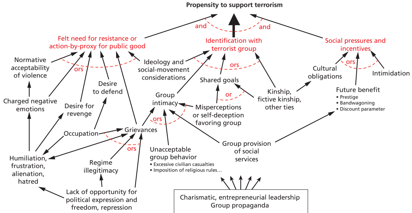
Figure 2.5 The Original Factor Tree for Public Support
