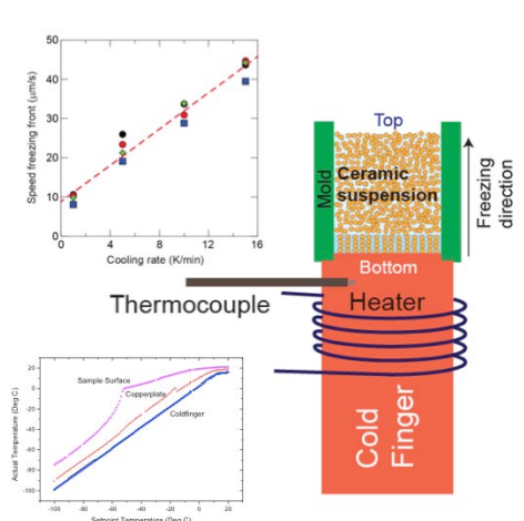
Figure 1. Freeze casting set-up. A teflon mould is filled with a ceramic suspension and placed on a cold finger that can be cooled at controlled rate (between 0 to 15 °C/min) to promote directional freezing. The speeds of the freezing front vary between 10 and 50 μm/s. A set of thermocouples can be used to record the temperature evolution in different locations in the mould and provide basic data needed to model the freeze casting process.
