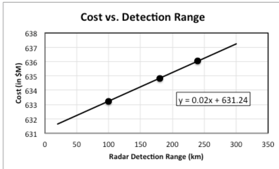
Figure 21. Cost vs. Detection Range Graph
