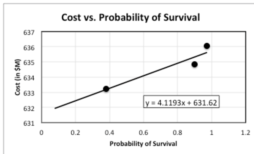
Figure 22. Cost vs. Probability of Survival Graph
