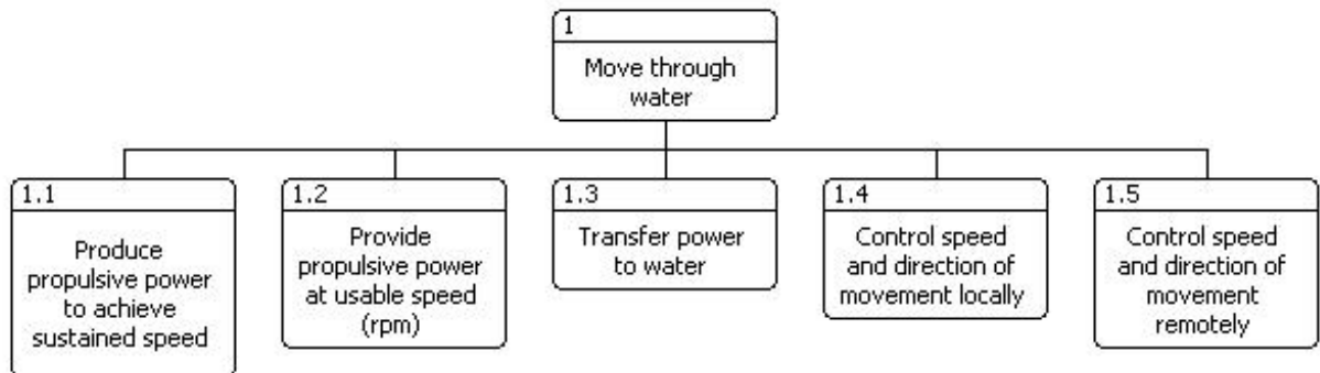
Figure 23. Second-level Functional Decomposition of Function 1
