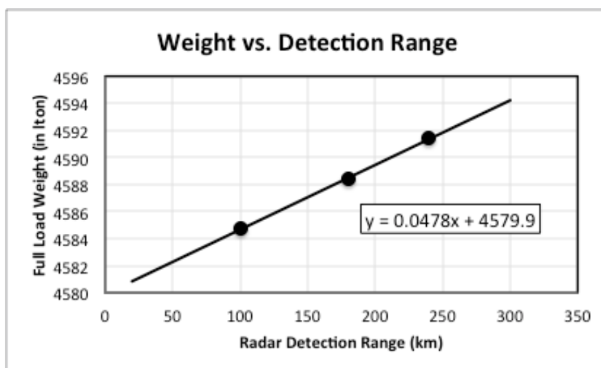
Figure 19. Weight vs. Detection Range Graph
