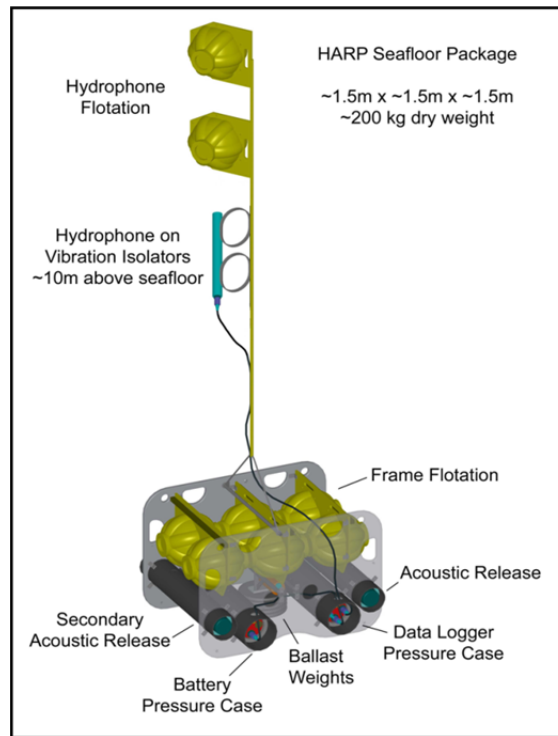
Figure 1. High-frequency Acoustic Recording Package (HARP) seafloor package. The HARP device is composed of three main components: a data acquisition system, a hydrophone sensor and instrument packaging. (From Wiggins and Hildebrand 2007).
