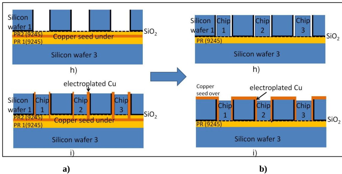
Figure 8. Amended process flow steps to account for Cu seed placement: (a) underneath the template and (b) on top of the template.
