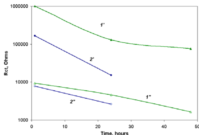
Fig. 7.6. Time dependencies of charge transfer resistance R_{ct} (1', 2') and solution resistance R_e (1'', 2'') for chromate containing (1', 1'') and uninhibited polyurethane coatings (2', 2'').
