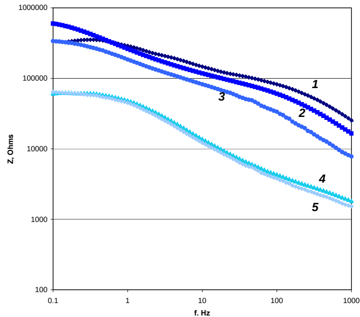
Fig. 9.1. Bode impedance diagrams of D16T alloy flat samples with uninhibited polyurethane coatings after 3 hours (1), 24 hours (2), 48 hours (3) and 120 hours (4) exposure in acid rain solution.
