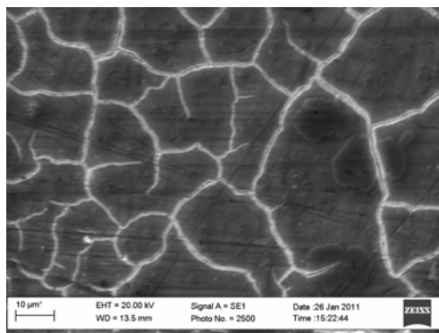
Fig. 4.20. Scanning electron image of surface film on aluminum alloy after its exposure in corrosion solution with phosphate/zeolite composition (phosphate/zeolite ratio - 0.66 g/l/ 0.34 g/l)
