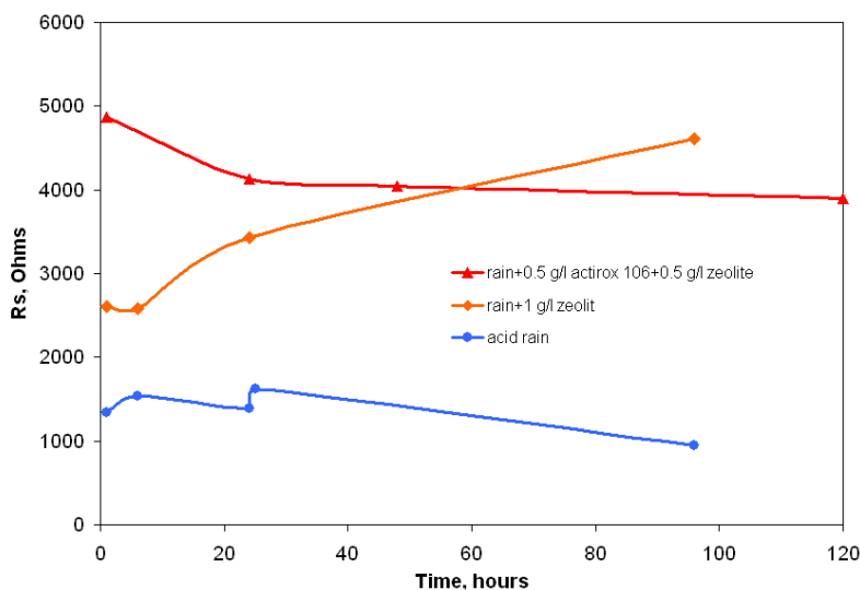
Fig. 4.14. Time dependencies of solution resistance during exposure of D16T alloy in inhibited acid rain.
