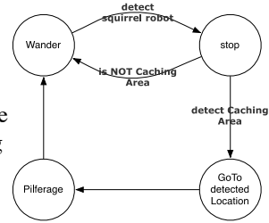
Fig 3. FSA for the Competitor robot
