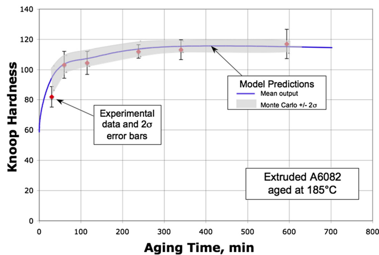
Figure 7 Comparison of experimental and modeling validation results for the MatLab Implementation of the Myhr precipitation model.
