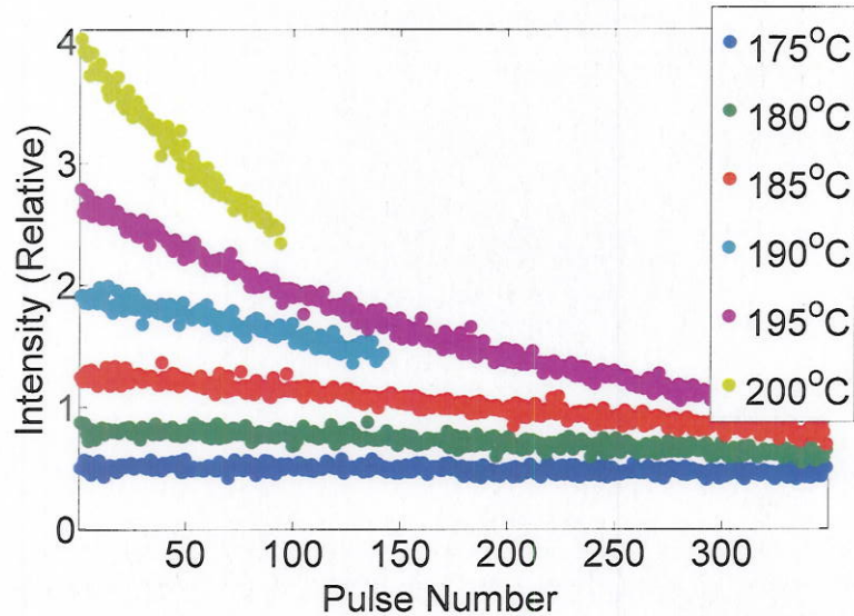
Figure 68: PTL at constant temperature. The pulse length was 50 ms. The temperatures of the pulses for different curves were 175, 180, 185, 190, 195 and 200°C.
