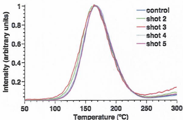
Figure 66 - Thermoluminescence glow curves of Al 2 O 3 :C before and after explosion with PETN charges. The data were collected using a linear heating ramp of approximately 0.9 °C/sec.
