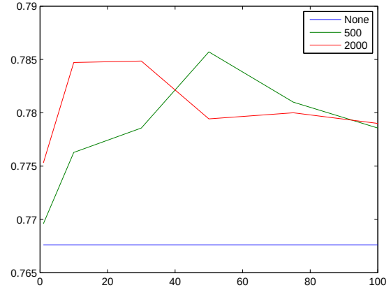
Figure 4: Average results of Reweighting among all 7 speakers when the amount of speaker specific data is 0, 500, 2000
