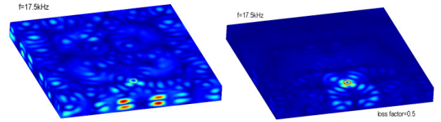
Figure 6: Stationary pattern of the total displacement of the WebCore panel at PZT frequency f=17.5\text{kHz} . The hole size 1/4 in is located at the center and PZT on a distance 10cm from the hole. Right plot is simulated for the same parameters but for 0.5 core loss factor.
