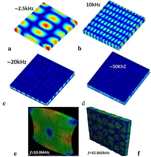
Figure 4: Shapes of eigenmodes for foam core panel – a-c, and honeycomb sandwich panel – e,f. At higher frequencies ( f \geq 10 kHz, for foam core and 30 kHz honeycomb panel), practically all normal modes are localized in the core, and facesheets practically do not respond.
