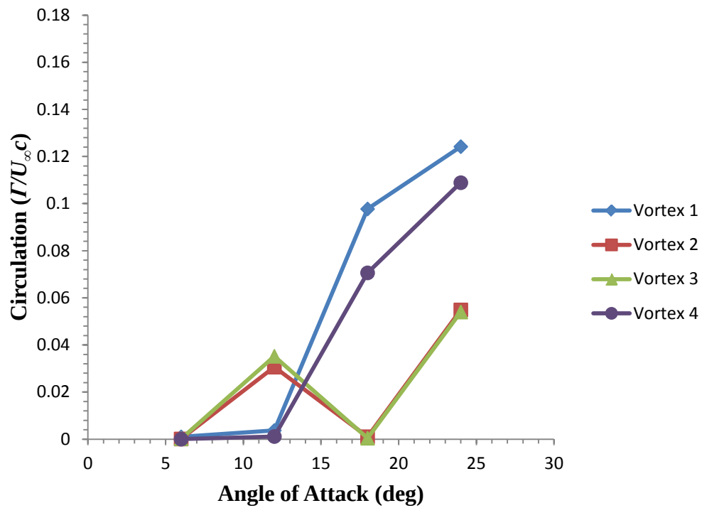
Figure 64. \Gamma as a function of \alpha at the chordwise location of x/c = 0.36 at U_\infty = 4.5 m/s.
