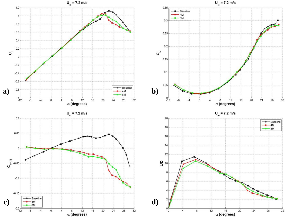
Figure 80. Effect of protuberance wavelength on the load characteristics of cavitating hydrofoils with a protuberance amplitude of A = 0.05 : a) lift coefficient, b) drag coefficient, c) pitching moment coefficient, d) lift-to-drag ratio.
