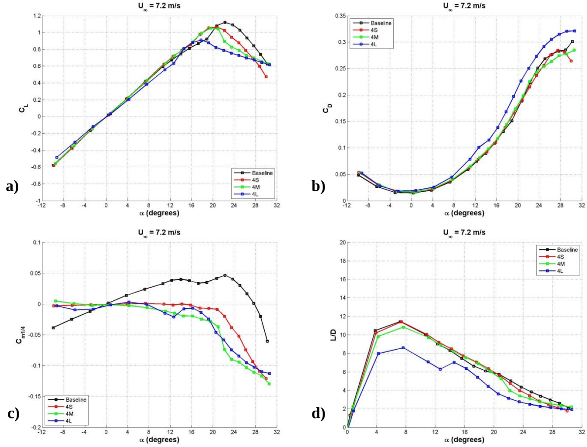
Figure 77. Effect of protuberance amplitude on the load characteristics of cavitating hydrofoils with a protuberance wavelength of \lambda = 0.50 c: a) lift coefficient, b) drag coefficient, c) pitching moment coefficient, d) lift-to-drag ratio.
