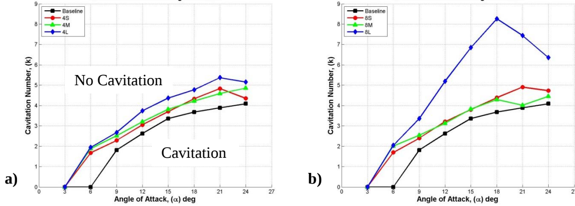
Figure 83. Incipient cavitation number of finite-span rectangular modified hydrofoils as a function of angle of attack: a) \lambda = 0.50 c , and b) \lambda = 0.25 c .
