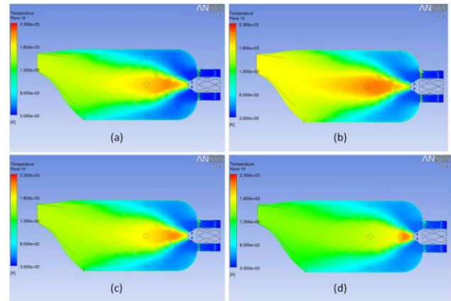
Figure 4. Temperature profiles of flames at the leanest equivalence ratio that will sustain a quality flame ( >95\% burned). A) no reforming, equivalence ratio 0.6, b) 5% of fuel reformed, equivalence ratio 0.6, c) 10% of fuel reformed, equivalence ratio 0.5, and d) 20% of fuel reformed, equivalence ratio 0.4.
