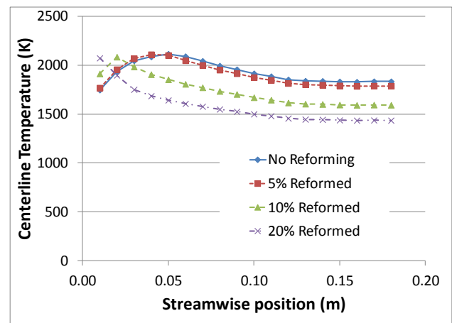
Figure 5. Axial temperature distribution in the leanest case allowing full combustion for each level of reforming: With no reforming, this lean equivalence ratio is 0.65, for 5% reformed it is 0.6, for 10% it is 0.5 and for 20% reformed it is 0.4
