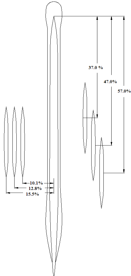
Figure 4: Sidehull Positions
