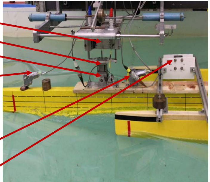
Figure 9: Model Instrumentation
