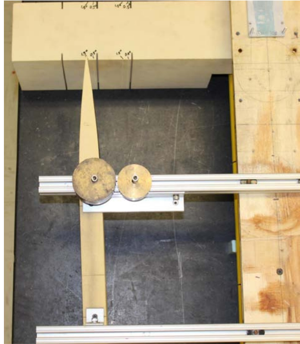
Figure 6: Splayed Sidehull Using Indexing Block
