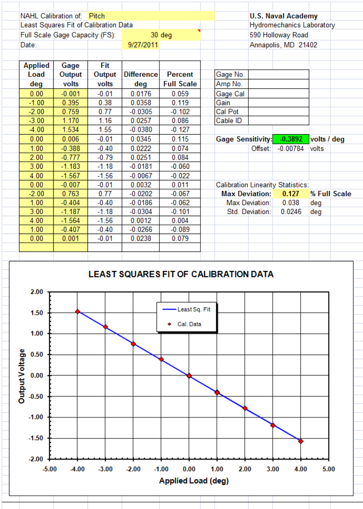
Figure 26: Pitch Pivot Gauge
