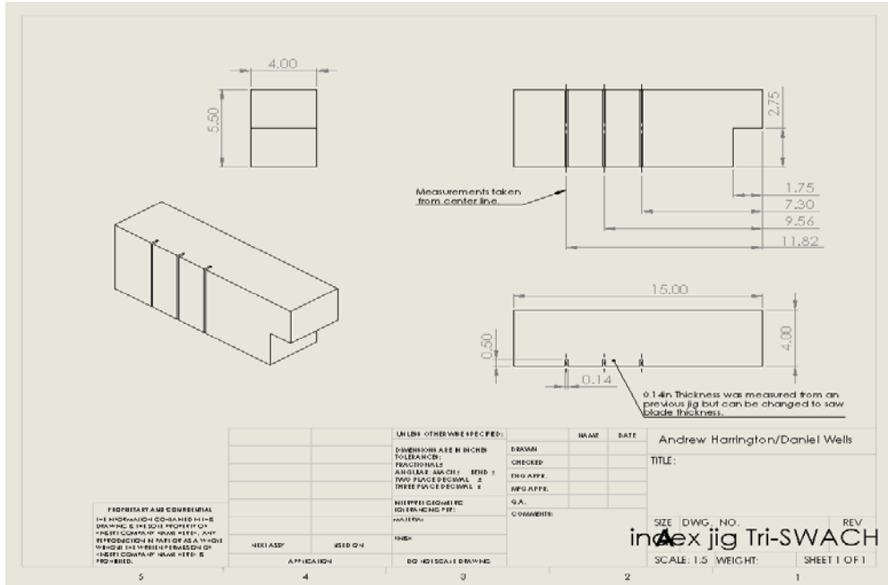
Figure 20: Solid Works Drawing Of Indexing Block
