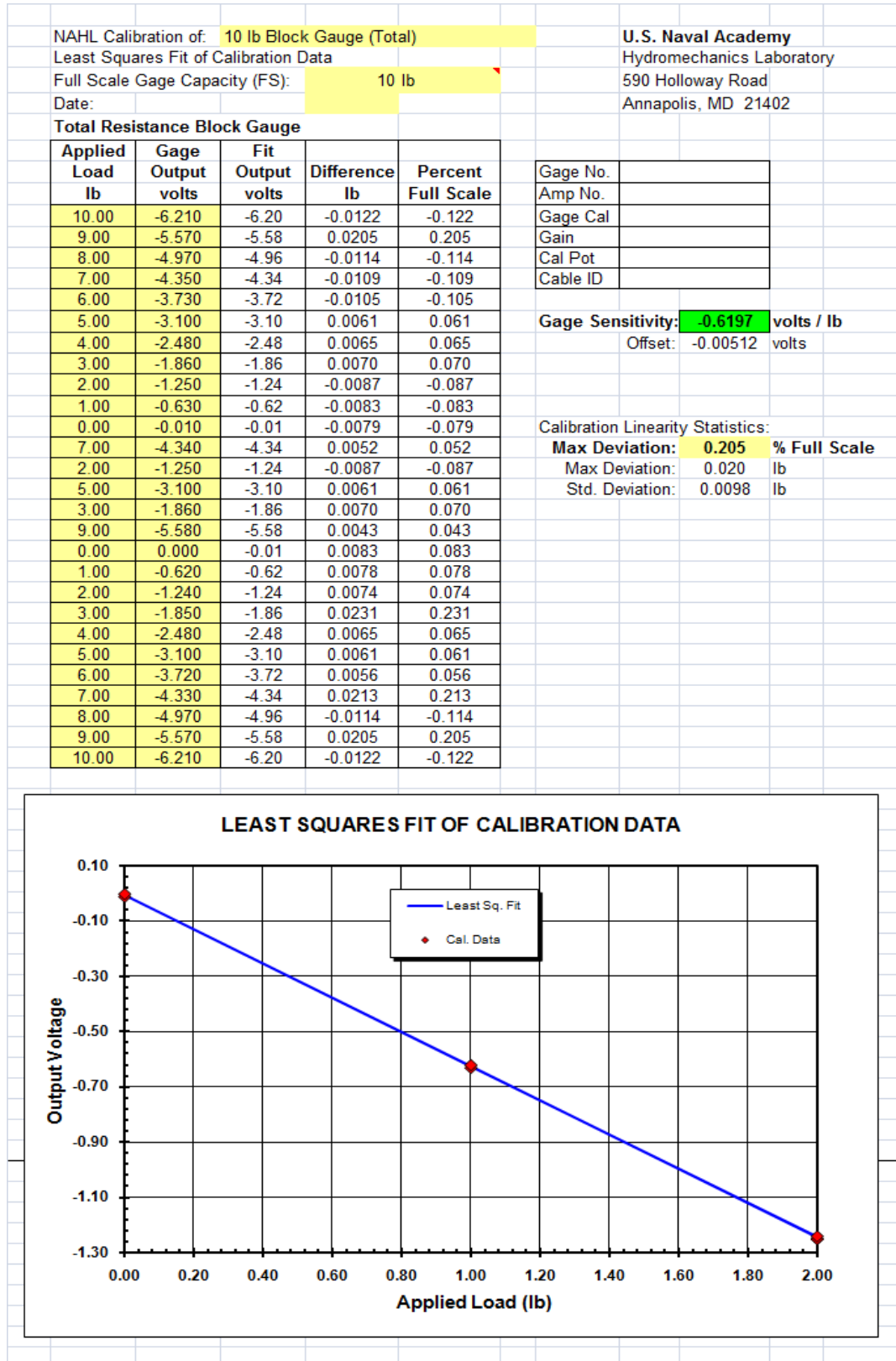
Figure 27: Total Resistance Block Gauge Calibration
