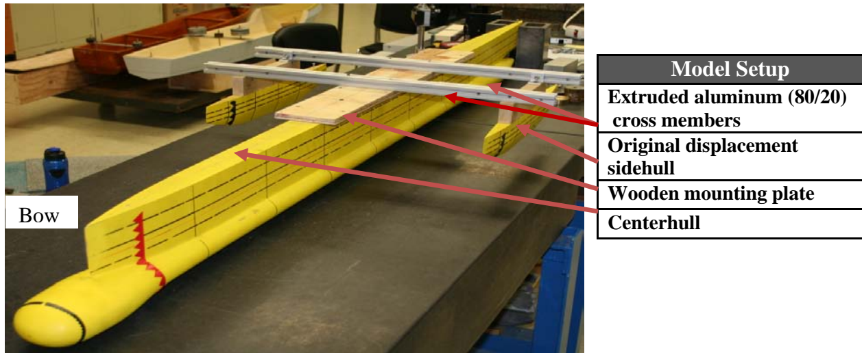
Figure 3: Tri-SWACH Model
