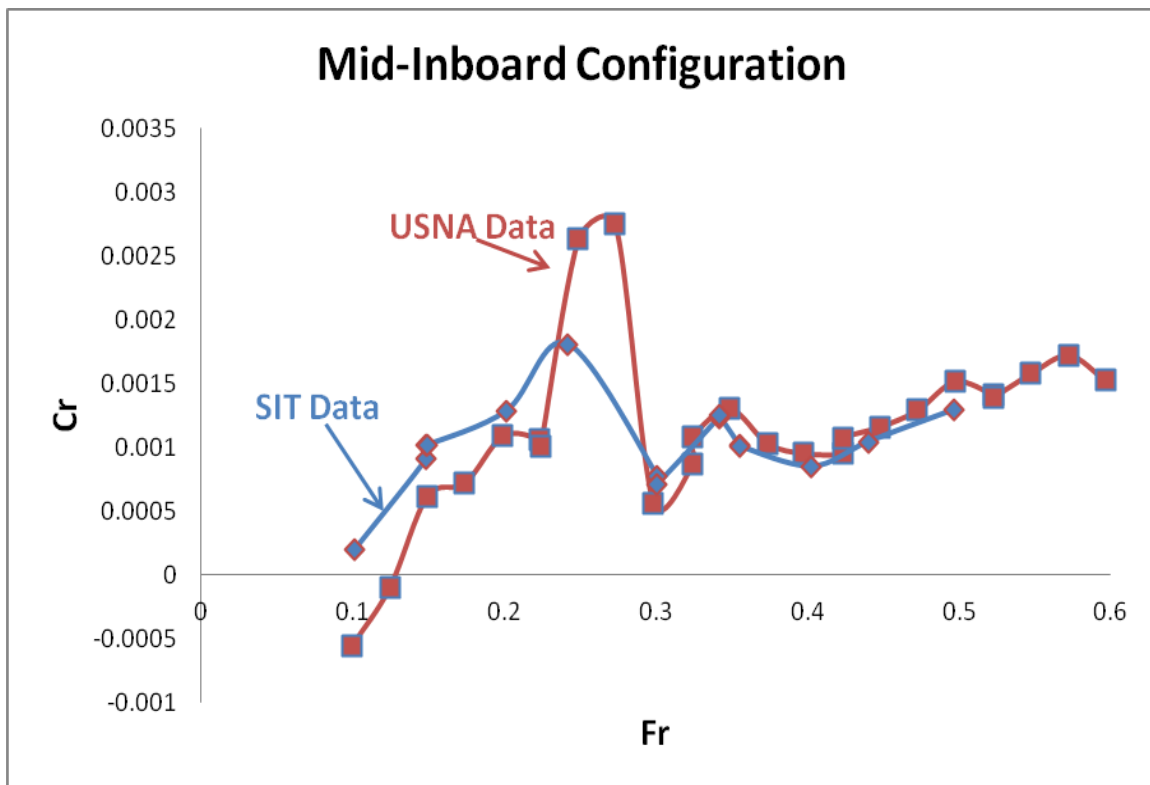
Figure 12: Calm Water Towing Tank Correlation for Mid-Inboard Location
