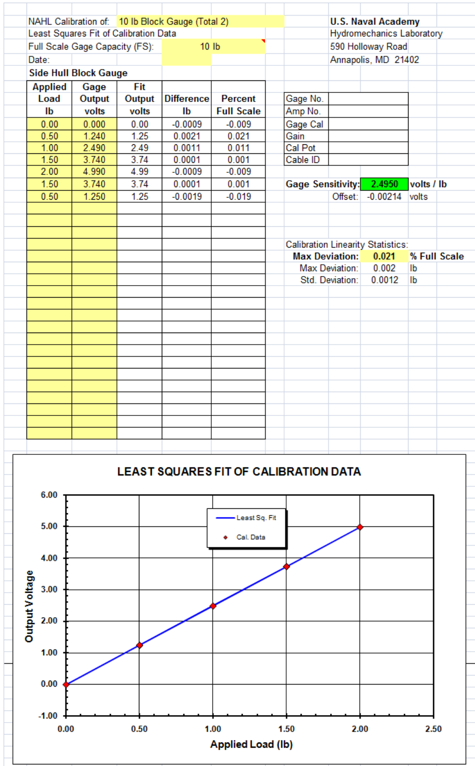
Figure 28: Side Hull Block Gauge Calibration
