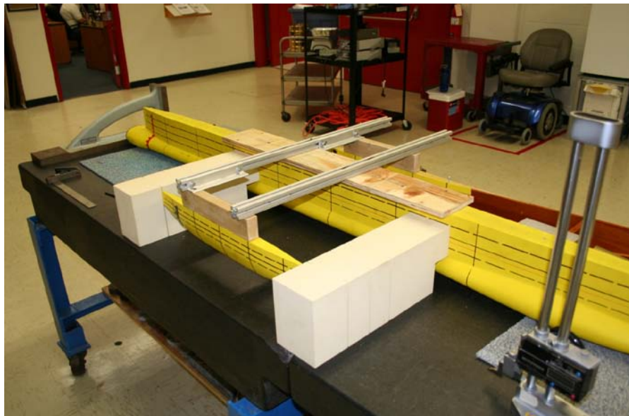
Figure 21: Model Setup Using Indexing Blocks
