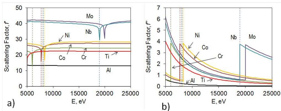
Figure 1. X-ray scattering factors (a) f' and (b) f'' for Al, Co, Cr, Mo, Nb, Ni and Ti in the X-ray energy range of 5000 to 25000 eV and Q = 0^\circ [36]. The vertical lines correspond to the energies used in this work.
