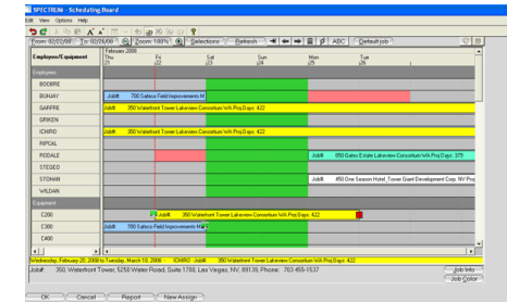
Scheduling Problems
