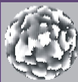
Target-return speckle field phase
