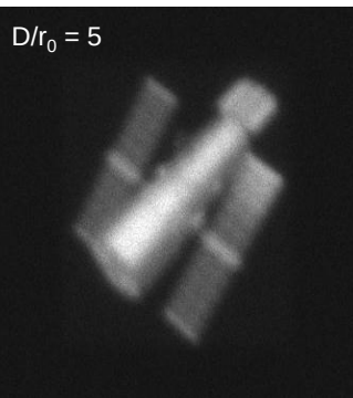
Good Seeing Terminator
