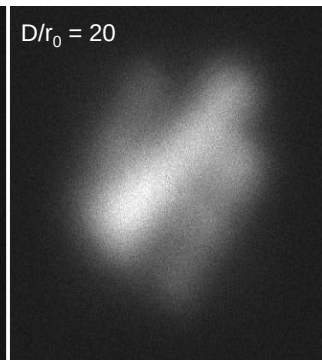
Marginal Seeing Terminator
