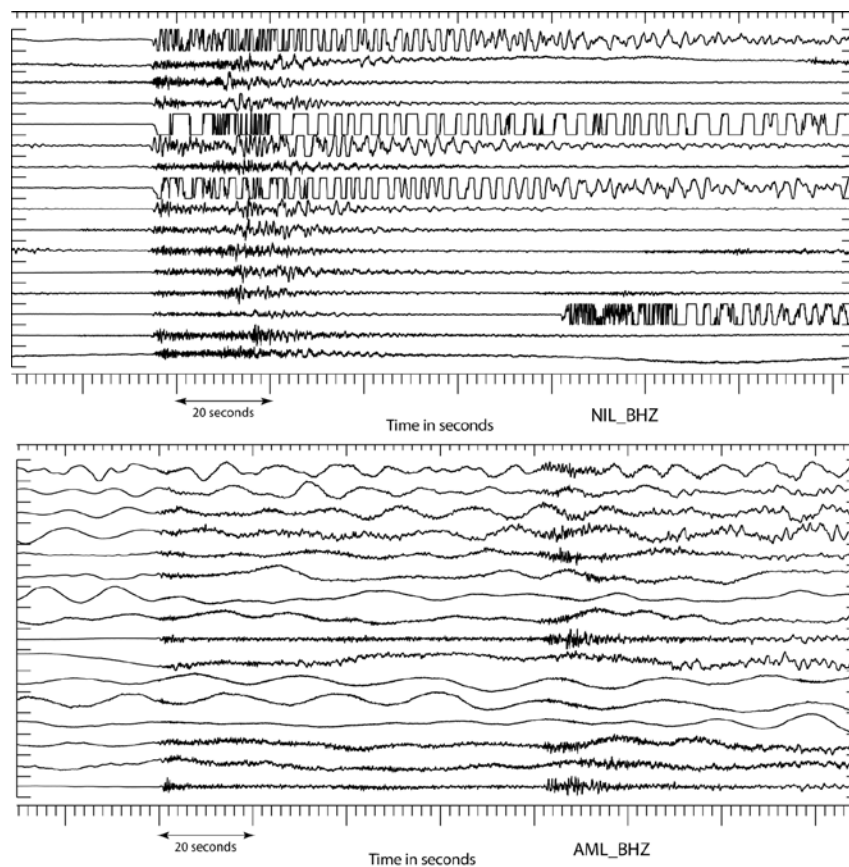
Figure 4. Unfiltered waveforms from NIL (Nilore, Pakistan: distance ~1 degree) and the AML station of KNET (distance ~9 degrees) for a selection of aftershocks from the October 8, 2005 Kashmir earthquake. Note that the dynamic range is exceeded for many of the signals at NIL.
