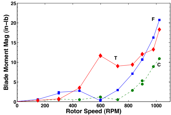
Figure 43. The effect of rotor speed on blade moments (B1 root), 2° elevon oscillation – 7 Hz.
