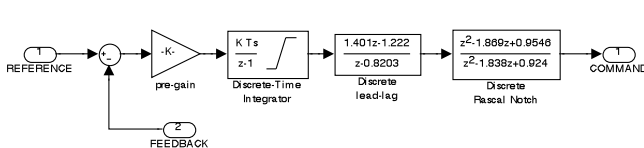
Figure 18. Classical controller block diagram.
