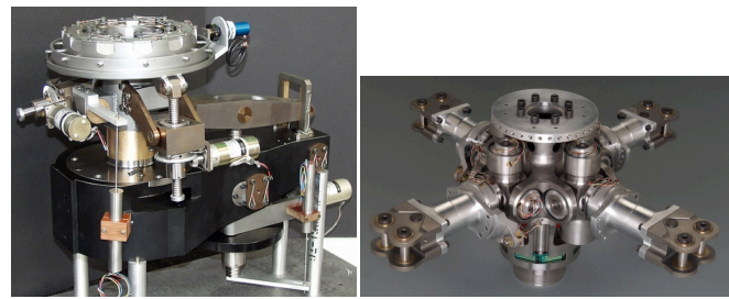
Figure 11. a) Swashplate and b) articulated hub.
