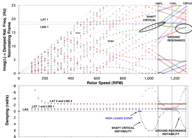
Figure 31. Aeromechanical stability ( b=2 ), unbraced.
