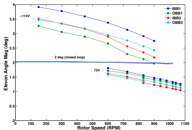
Figure 37. The effect of rotor speed on elevon deflection – 7 Hz response to 7 Hz voltage, for two open loop cases (75V and \sim 115 V) and one closed loop case ( 2^\circ ).
