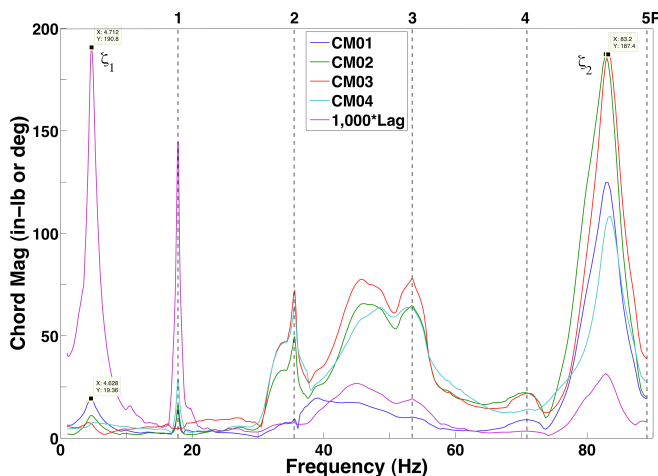
Figure 47. FRF magnitudes of the chord bending moment at four STAs and lag angle, 1070 RPM.
