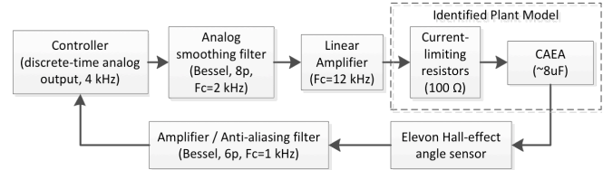
Figure 15. Control system block diagram.
