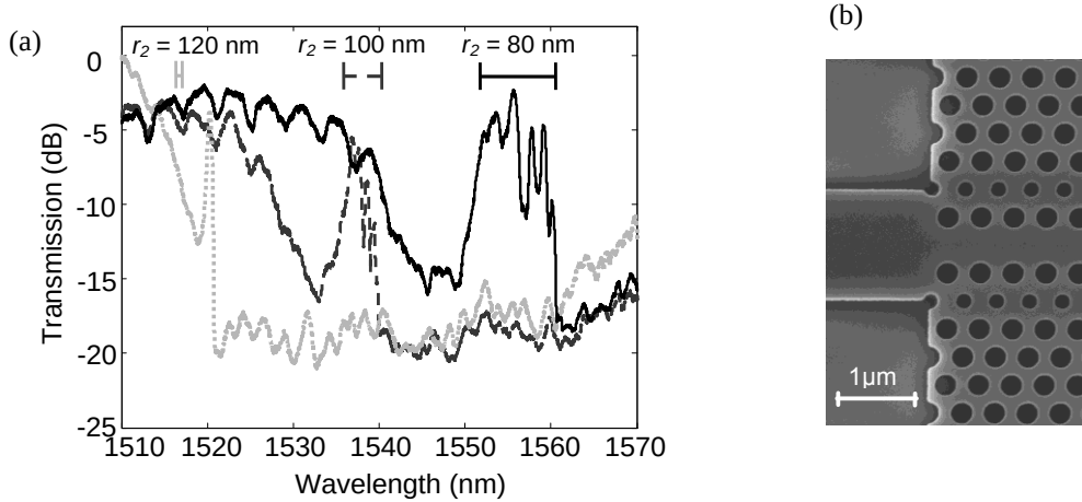
Figure 2. Transmission spectra of W1 PCWs fabricated on SOI with the silicon thickness of 250 nm with a=400 nm and r_1=0.3a=120 nm. The transmission spectrum for PCWs with r_2=120 nm, r_2=100 nm and r_2=80 nm are measured and shown by dotted, dashed and solid curves, respectively. (b) Scanning electron micrograph of the fabricated device at the interface of the input ridge to PCW.
