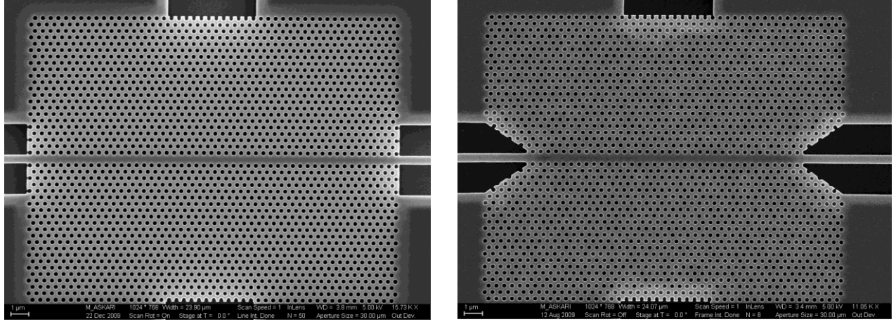
Figure 4. SEM image of fabricated butt coupler (left) and air wedge coupler (right).
