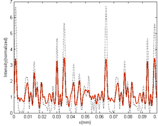
Fig. 2. The intensity of a plane wave scattered by particles and normalized by its value on the axis vs. radial distance from the optical axis: with turbulence (solid curve); without turbulence (dotted curve).
