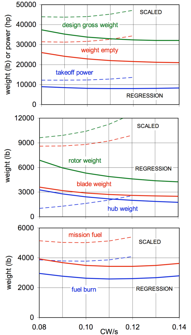
Figure 21. Variation of civil aircraft design with blade loading C_W/\sigma (disk loading 16 lb/ft² for scaled rotor weight model, 12 lb/ft² for regression rotor weight model).
