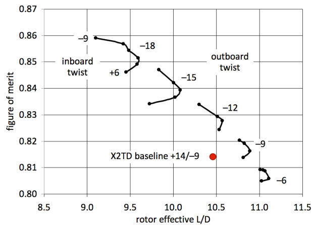
Figure 13. Influence of twist on calculated hover and cruise performance of the X2TD.
