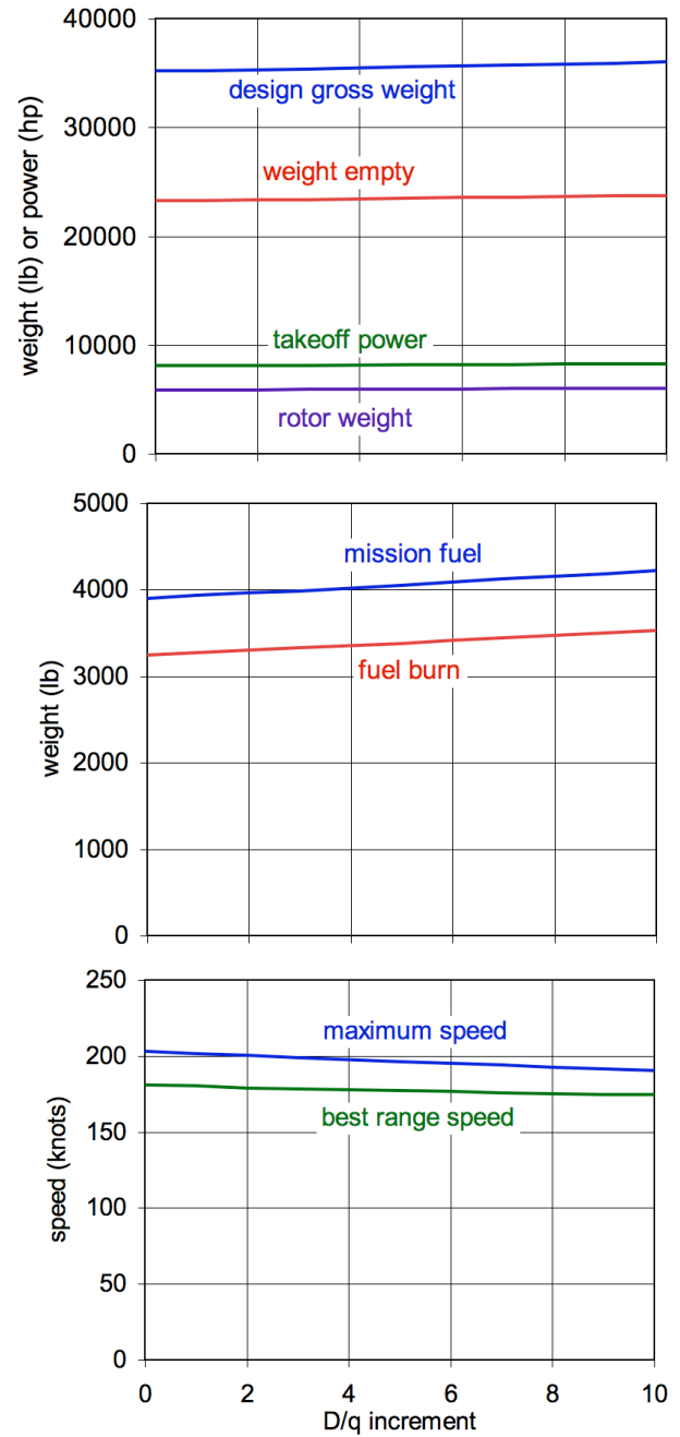
Figure 37. Influence of aircraft drag increase ( \Delta D/q , ft 2 ) on military aircraft with regression rotor weight model.
