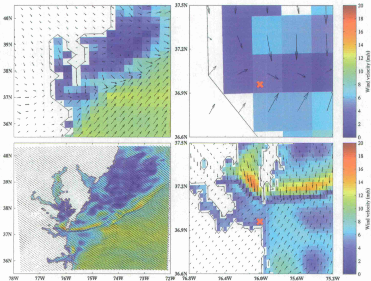
Fig. 12 The magnitude and direction of surface wind at hour 1 on 7 June 2010 from 27-km resolution operational COAMPS over the western North Atlantic shelf ( top left ) and southwest of the Chesapeake Bay, MD ( top right ). Triple-nested, 3-
