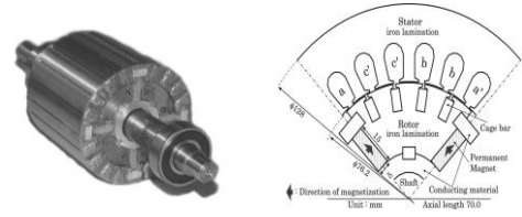
Fig.2: IPM Rotors for Line Start Motor [25].
