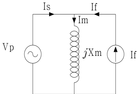
Fig 1. Norton's equivalent circuit of IPM Motor.
