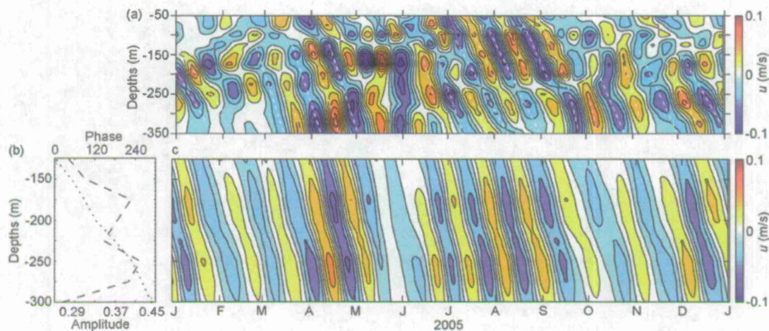
Fig. 6. Across-strait flow varying at periods of 20–40 days observed at Mak-West mooring in 2005 (a) and its orthogonal function approximation (b and c). Dashed lines in (a) show phase lines. Dashed and dotted lines in (b) show the 1st eigenvector and its relative phase that represents 50% variance of (a). (c) Reconstructed across-strait flow for the 1st mode.
