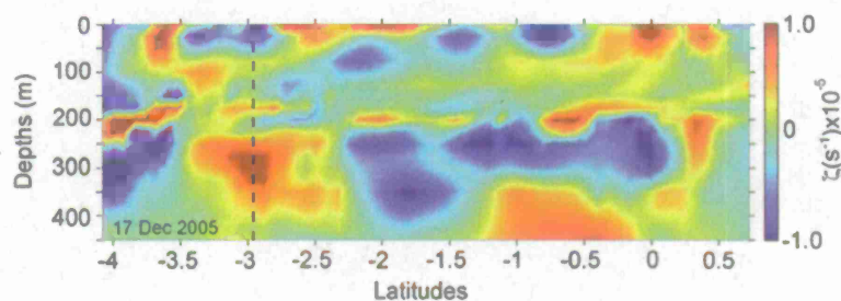
Fig. 12. The model \xi' plot for several depths along a transect in Makassar Strait shown in Fig. 1, simulated on 17 December 2005. The \xi' time series are computed using horizontal velocities for intraseasonal timescales. The dashed line indicates the latitude of the mooring location in the Labani Channel.
