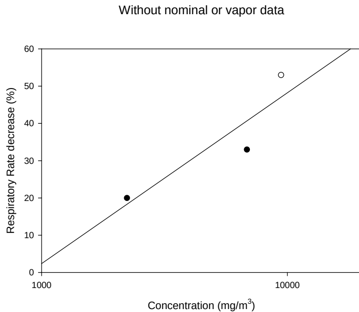
Figure 11. RD 50 Recalculation for FT Jet Fuel
