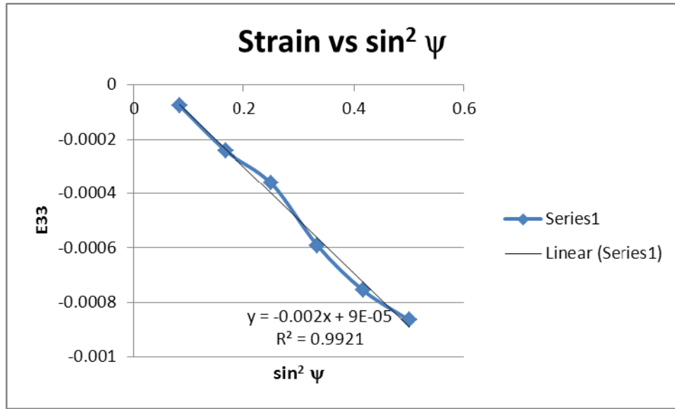
Figure 44. Strain versus. \sin^2\psi .
