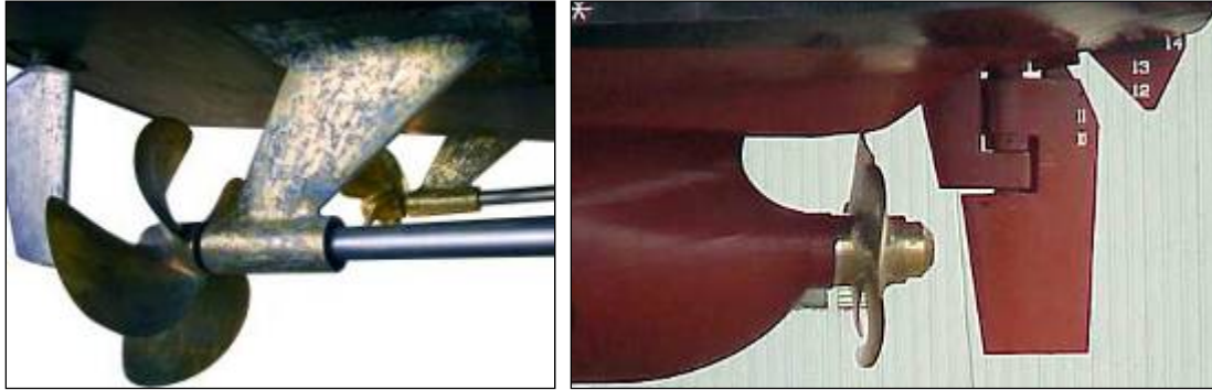
Figure 36. Different Types of Propulsion Design (From [90])
