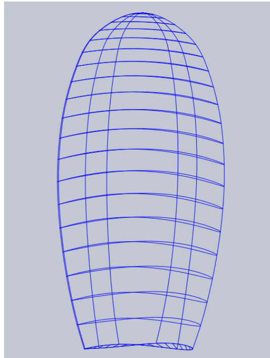
Figure 57. Geometry of the Propeller Blade for Case 2
