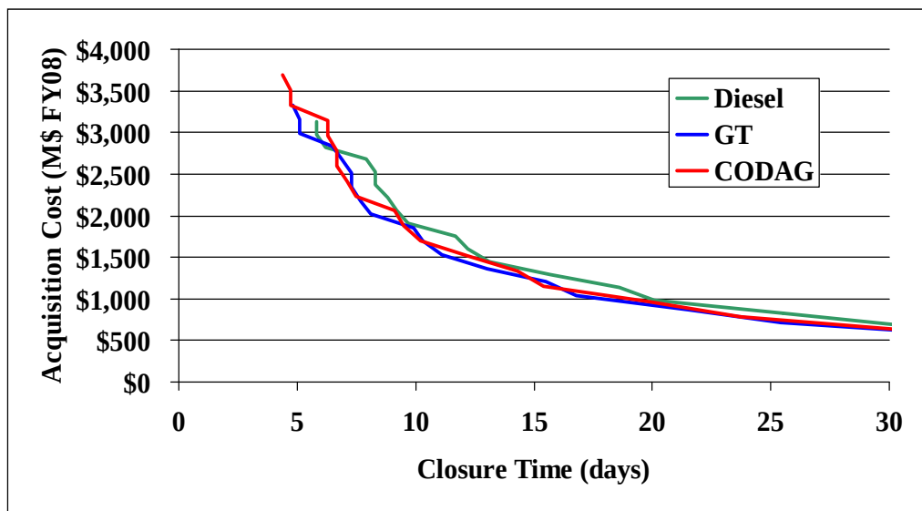
Figure 4. Propulsion System Trade-Off Between Closure Time and Acquisition Cost
