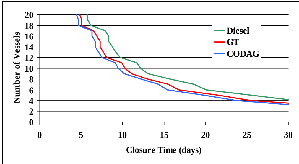
Figure 3. Propulsion System Trade-Off Between Closure Time and Number of Vessels
