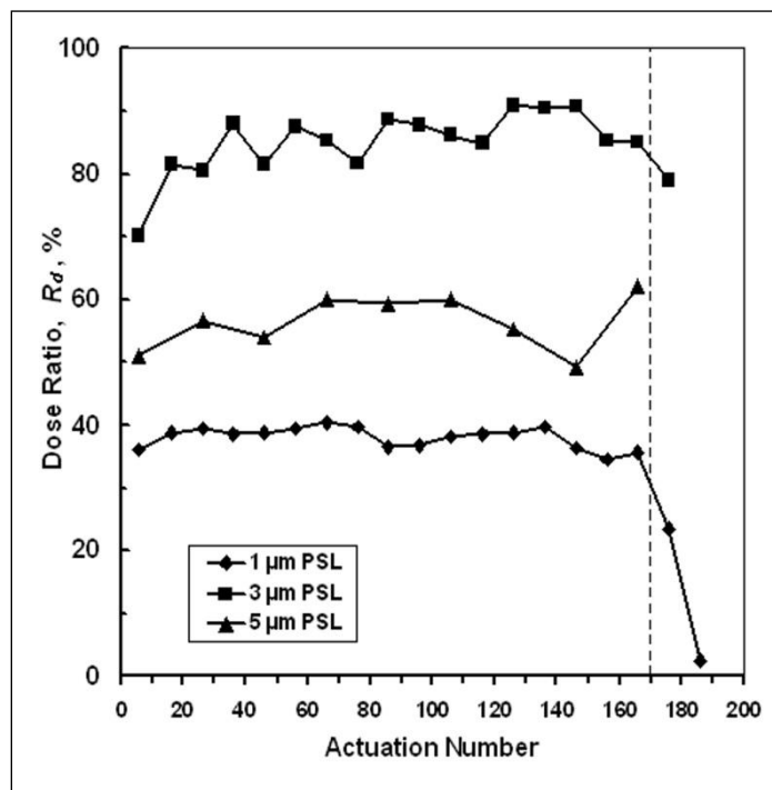
Figure 4. Constancy of PSL doses with usage. Dose ratio is the actual mass of aerosol particles released per actuation divided by the calculated amount released per actuation. BioMDDs were used without actuators (configuration shown in Figure 2b). A dashed line is shown at 170 actuations, which represents the approximate limit of usefulness of a 10 mL canister fitted with a 50 \mu\text{L}/\text{actuation} metering valve.
