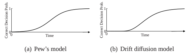
Figure 1: The evolution of the probability of the correct decision under Pew's and drift diffusion model. Both curves look similar and are sigmoid.
