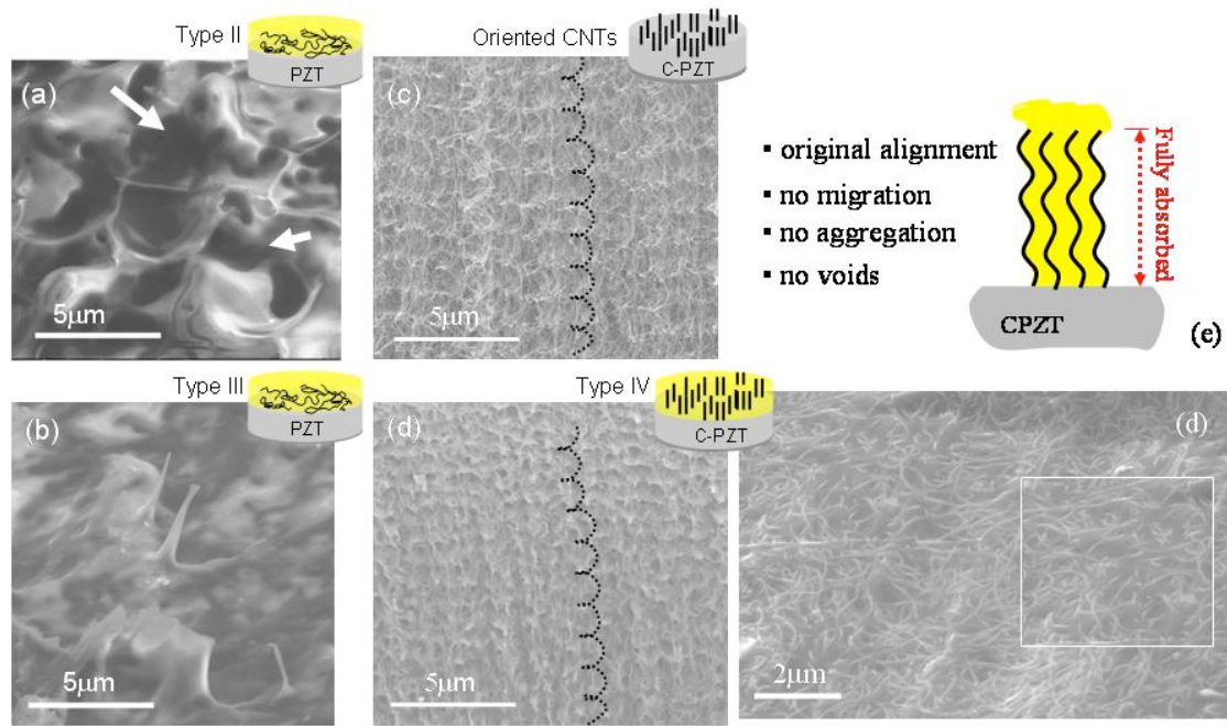
Figure 15. SEM images of the nanostructured bondlines used for the mechanical study: (a) adhesive mixed with random CNTs (Type II), (b) adhesive mixed with random CNTs (Type III), (c) side view of an oriented CNTs forest transferred onto a PZT surface (CPZT) before the embedding process. The wavelike configuration of the CNTs is highlighted. (d) side view of the CNTs forest (shown in (c)) embedded into the adhesive polymer (Type IV). After embedding, CNTs keep the same wavelike configuration (highlighted), (d) top view of the embedded CNTs forest, (e) schematic of the integration result for the case of oriented CNTs
