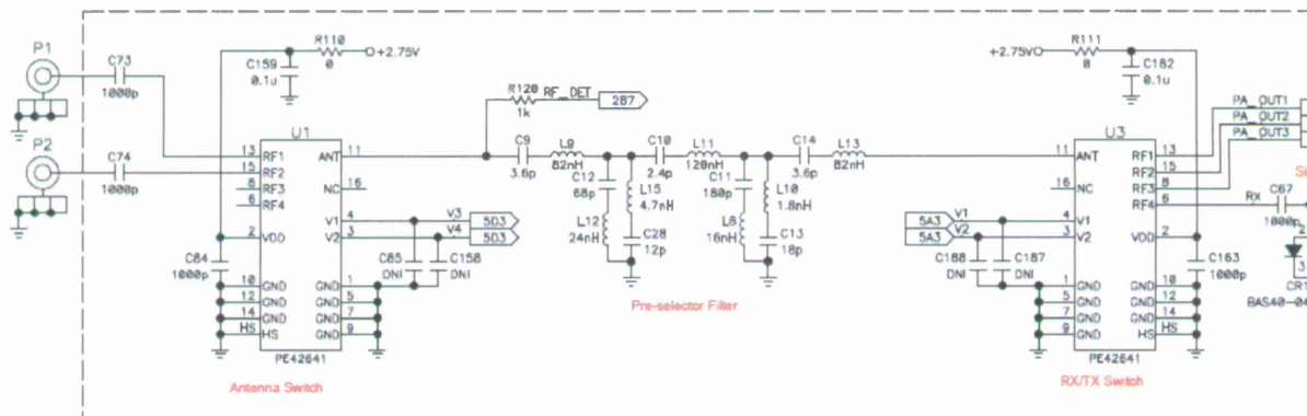
Figure 5. R.F. switches and pre-selector filter schematic
