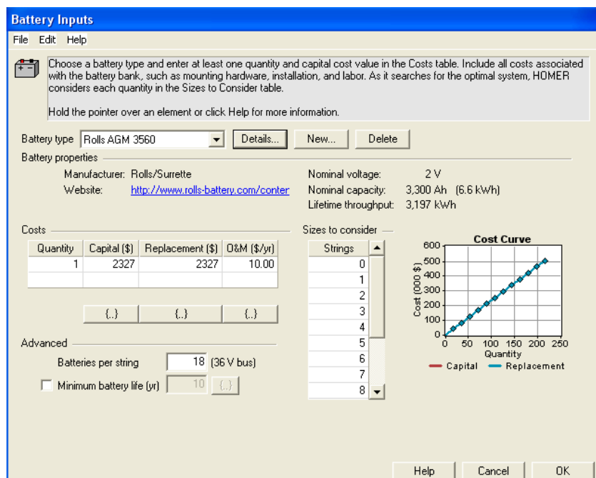
Figure 38. Battery cost data. (From: NREL, 2011)
