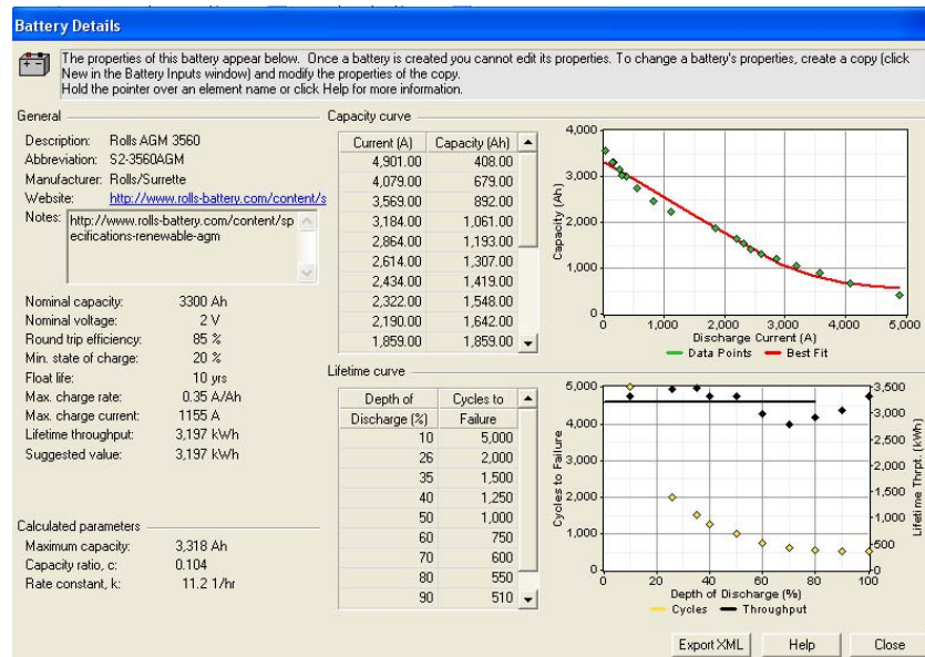
Figure 37. Battery input specifications. (From: NREL, 2011)
