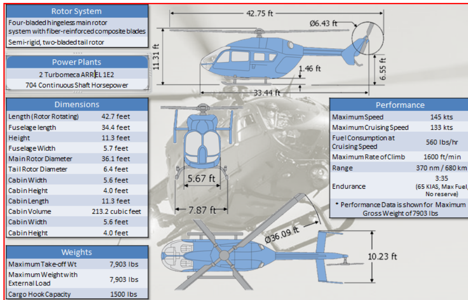
Figure 1. UH-72A LAKOTA 61
