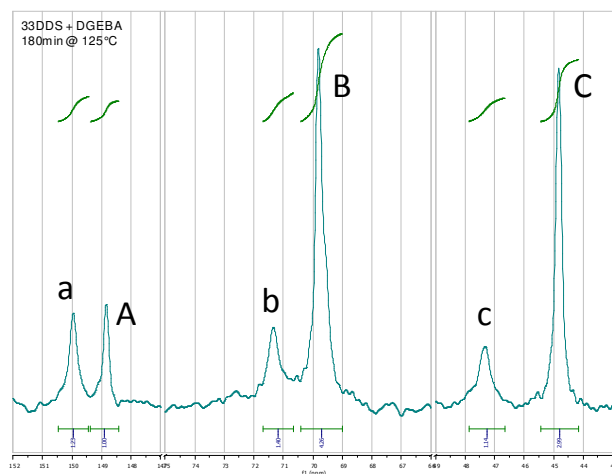
Figure 54. 33DDS and DGEBA after 180min at 125°C.
