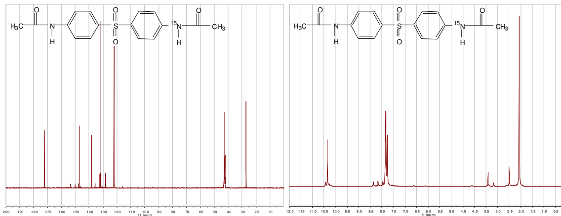
Figure 47. ^1\text{H} and ^{13}\text{C} NMR of ^{15}\text{N} 4,4'-di-n-acetylaminothiophenyl sulfone.
