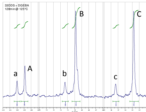
Figure 53. 33DDS and DGEBA after 128min at 125°C.
