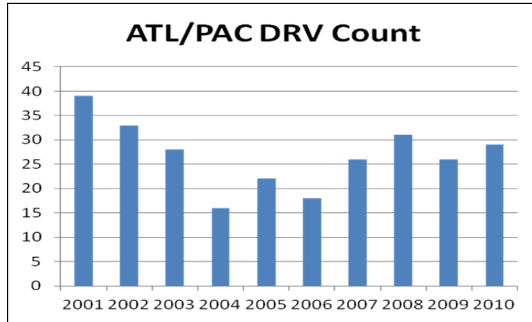
Figure 40. Combined ATL/PAC annual DRV histogram from 2001 to 2010.
