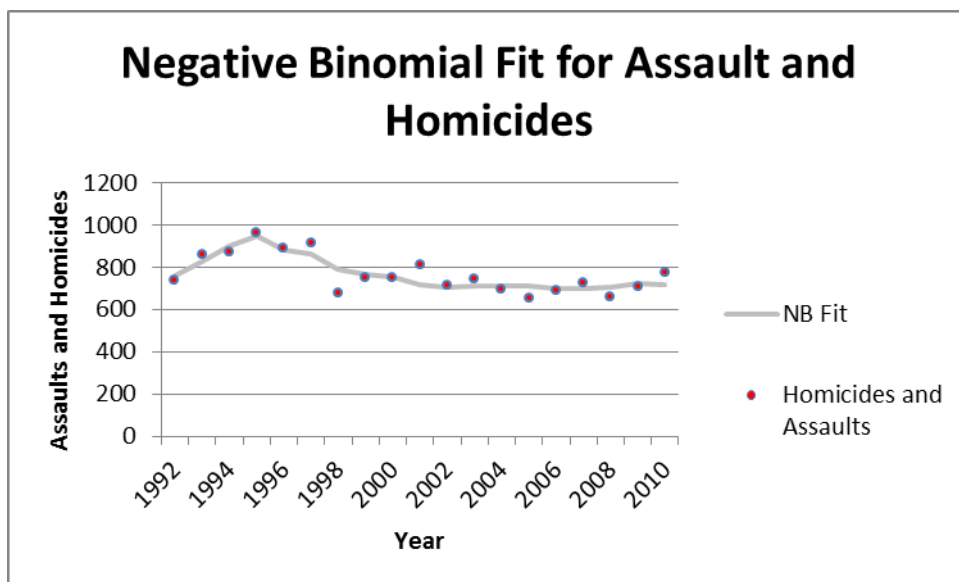
Figure 16. Negative Binomial Fit for Assault and Homicides
