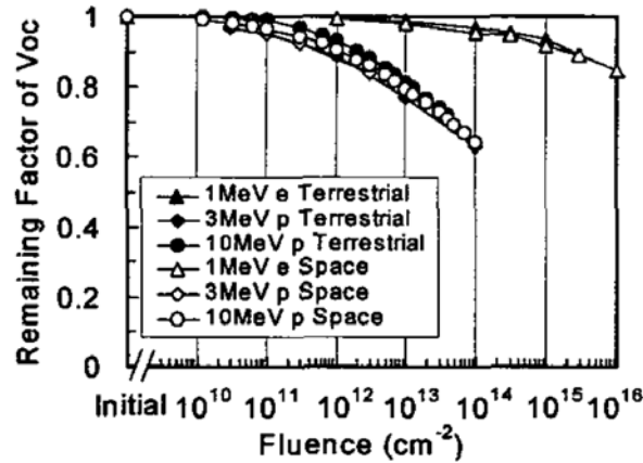
Figure 59. Remaining open circuit voltage after different levels of radiation. From [44].
