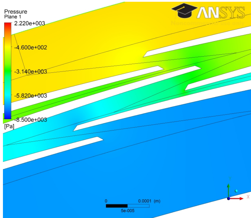
Figure 26. Minimum Pressure Ratio Two-Dimensional 2nd Design
