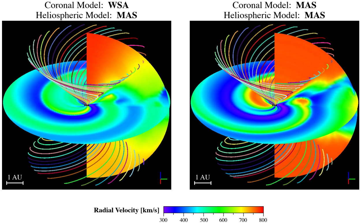
Figure 5. Heliospheric solutions computed out to 5 AU for CR2068 (March 19-April 16, 2008, the WHI interval). Both solutions were computed with the MAS heliospheric model. Velocity color maps in a meridional slice and the equatorial plane are shown, together with selected magnetic field lines. The case on the left used the WSA model for the interior coronal solution and specification of the inner heliospheric boundary condition. The case on the right used the polytropic MAS coronal model. The stream interfaces are sharper and the high-speed streams are faster when the MHD model is used for the coronal solution.
