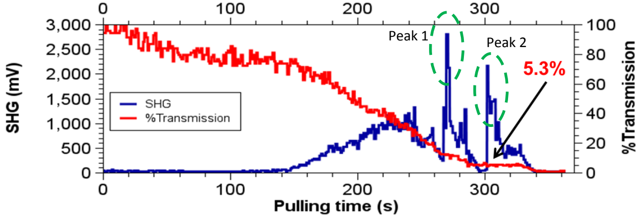
Fig. 10. The transmission of pump light (1294 nm) as well as SHG signal recorded in real time during fiber pulling. The schematic of experimental setup is shown in Fig. 9.
