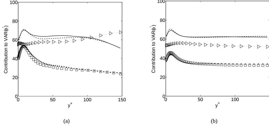
Figure 1: Percentage of VAR(\phi') for events with different conditions. Solid line, P(\widehat{\phi'^2} \geq k\phi^{+2}; \widehat{u'v'} < 0) ; -\cdot-\cdot- , P(\widehat{\phi'^2} \geq k\phi^{+2}; \widehat{\theta'v'} < 0) ; \cdot\cdot\cdot , P(\widehat{\phi'^2} \geq k\phi^{+2}; \widehat{u'v'} < 0; \widehat{v'} < 0) ; \square\square\square , P(\widehat{\phi'^2} \geq k\phi^{+2}; \widehat{\theta'v'} < 0; \widehat{v'} < 0) ; \triangleright\cdot\triangleright\cdot\triangleright\cdot\triangleright , P(\widehat{\phi'^2} \geq k\phi^{+2}; \widehat{\partial p'/\partial x} > 0) . (a) Channel flow; (b) Couette flow.
