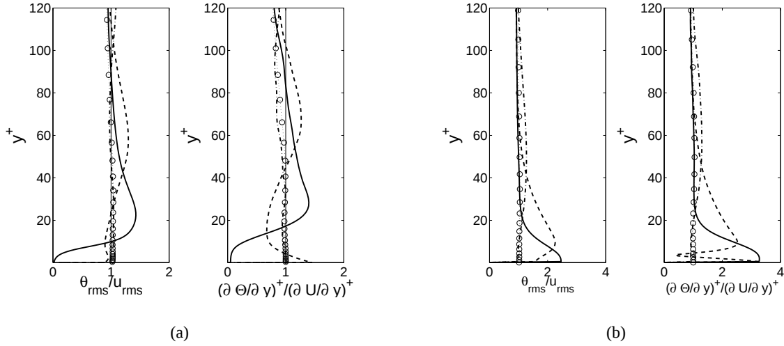
Figure 7: \theta_{rms}/u_{rms} and (\partial \Theta / \partial y) / (\partial U / \partial y) for channel flow perturbed with (a) blowing and (b) temperature step at the wall. \circ \cdot \circ \cdot \circ \cdot \circ , non-perturbed values. Solid line, on the slot; --- , W^+ ; -\cdot-\cdot-\cdot- , 5W^+ downstream.
