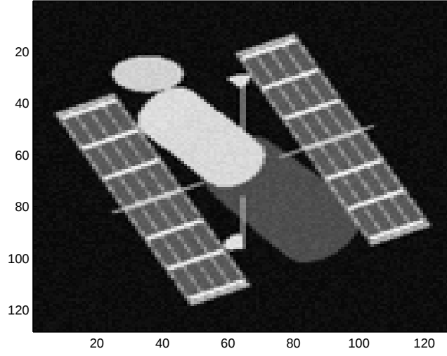
Figure 1: The spatial brightness distribution of the simulated HST in the middle spectral channel
